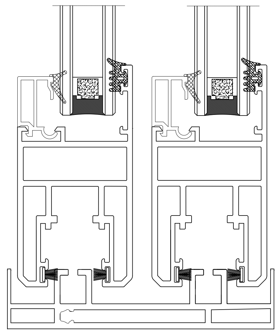
A SECTION DETAIL
